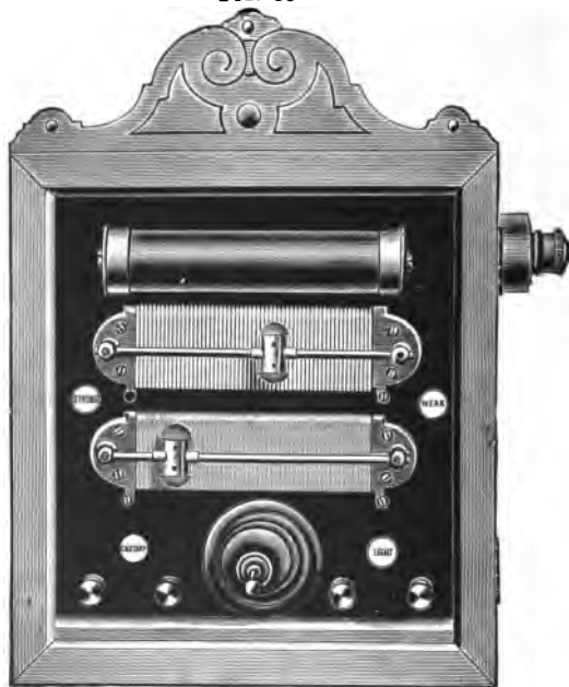
Transformer.
